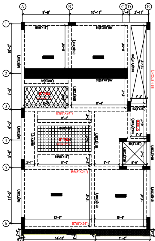
GROUND FLOOR ROOF FORMWORK LAYOUT
