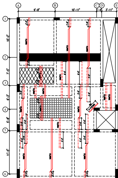
GROUND FLOOR ROOF SLAB REINFORCEMENT LAYOUT
