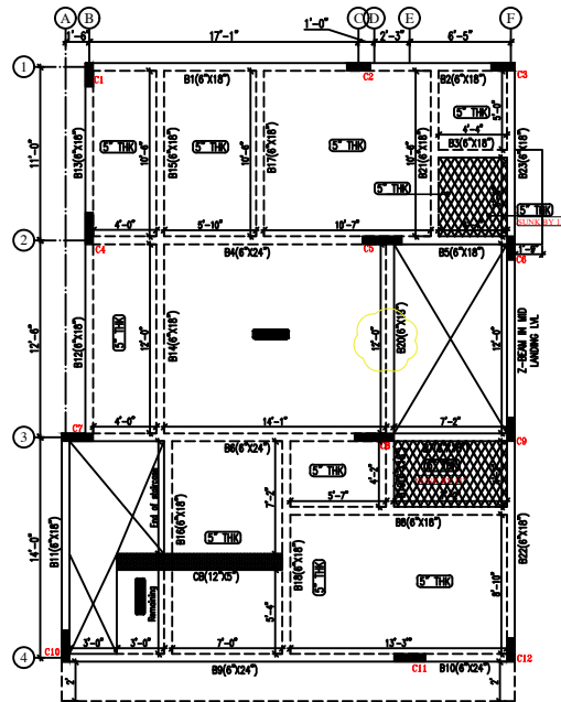
GROUND FLOOR ROOF FORMWORK LAYOUT
