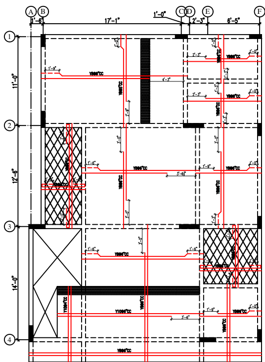
FIRST FLOOR ROOF SLAB REINFORCEMENT LAYOUT
