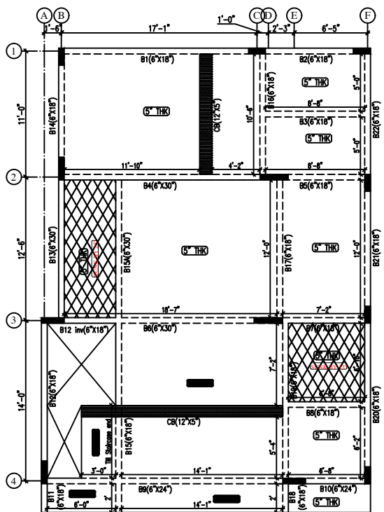
FIRST FLOOR ROOF FORMWORK LAYOUT
