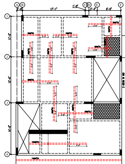
GROUND FLOOR ROOF SLAB TOP REINFORCEMENT LAYOUT
