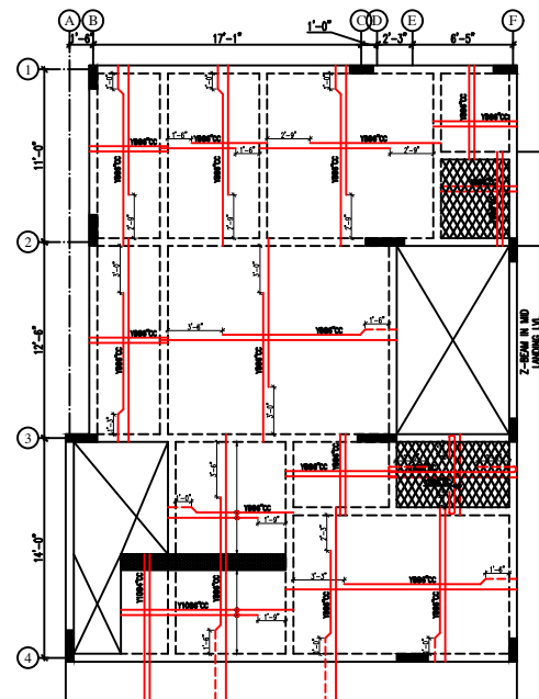
GROUND FLOOR ROOF SLAB BOTTOM REINFORCEMENT LAYOUT
