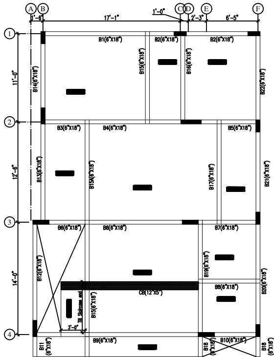
second floor roof formwork layout
